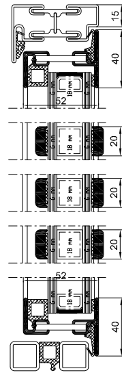
SECTION B-B
